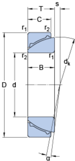
GAC 110 F Bearing 2D drawings and 3D CAD models
